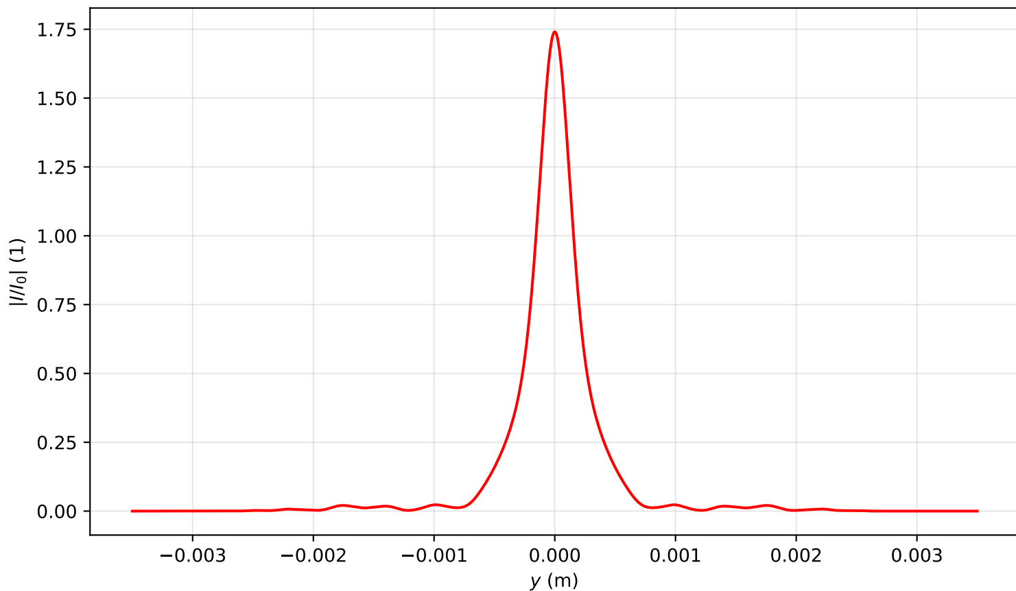
Intensity profile I(x=0, y, z=2.388)/I_0 , P_{in}=3.0P_{cr} , artificial time
